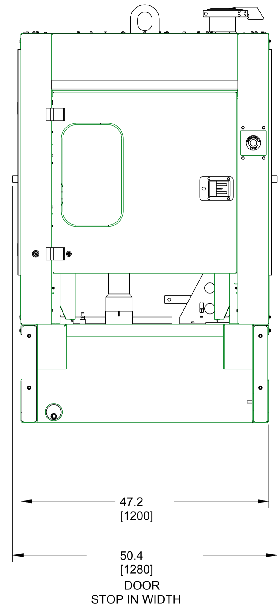
LESS RUNNING GEAR OPTION (CONTROLS VIEW)
