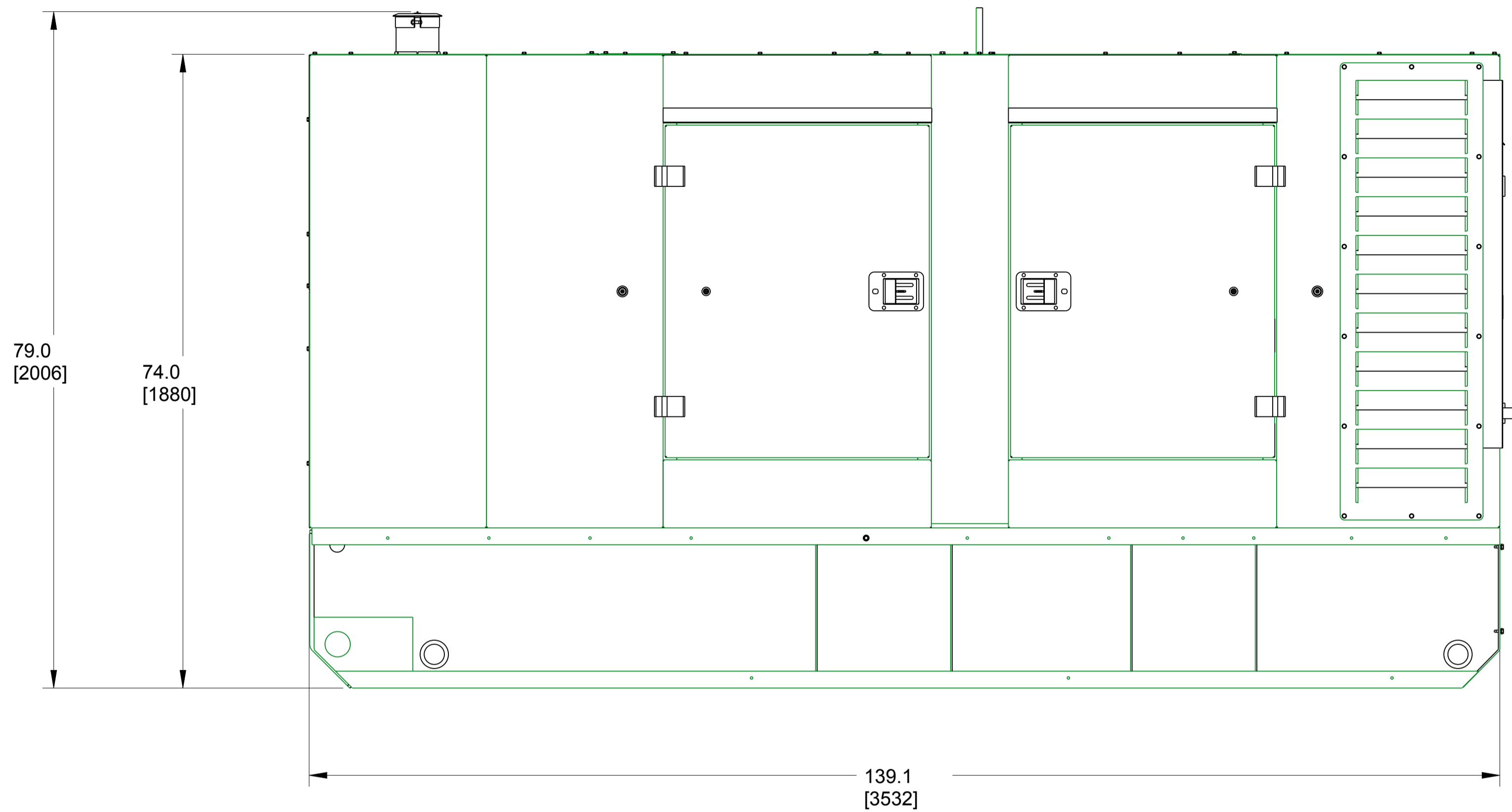
LESS RUNNING GEAR OPTION (LEFT VIEW)
