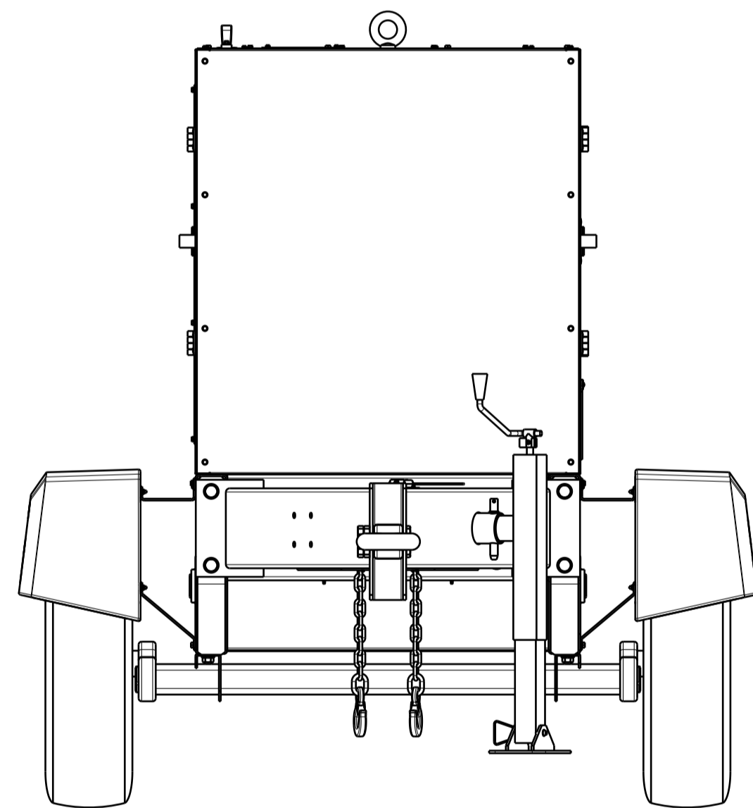
FRONT VIEW SEE SHEET 4 FOR ENLARGED VIEW
