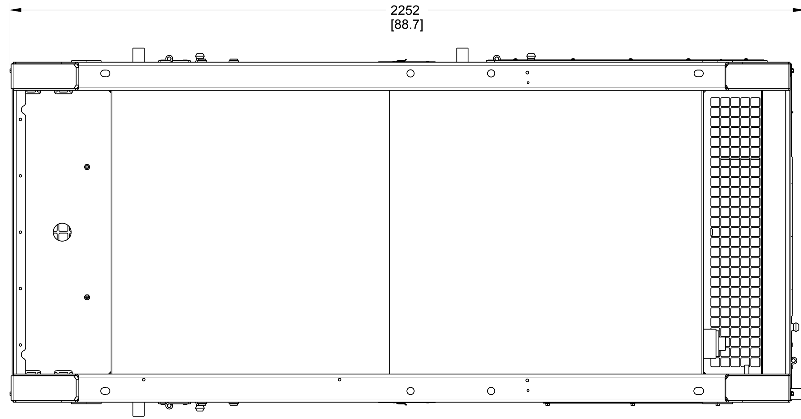
LESS RUNNING GEAR OPTION (BOTTOM VIEW)
