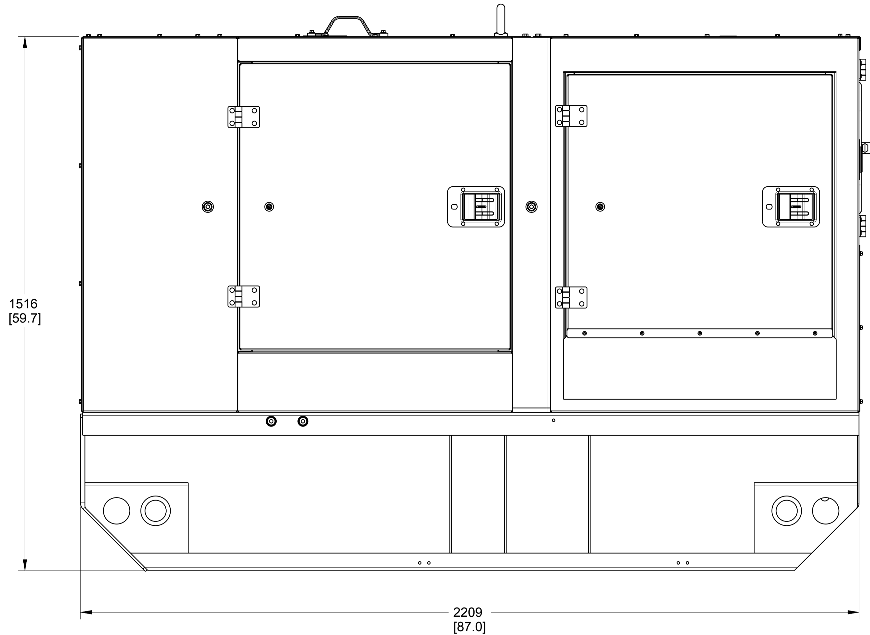
LESS RUNNING GEAR OPTION (STREETSIDE VIEW)
