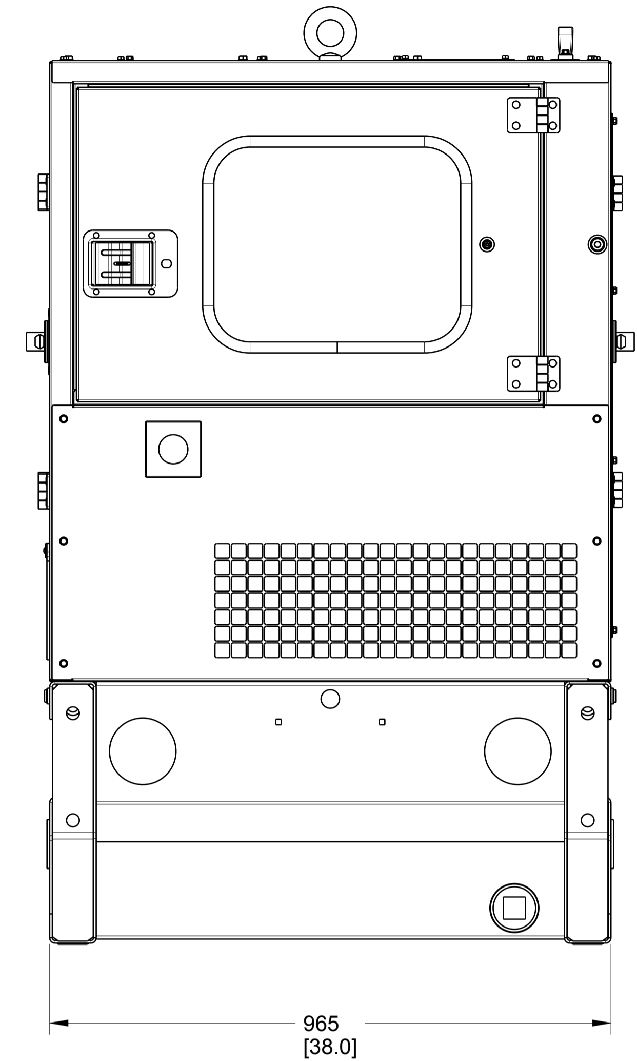
LESS RUNNING GEAR OPTION (CONTROLS VIEW)
